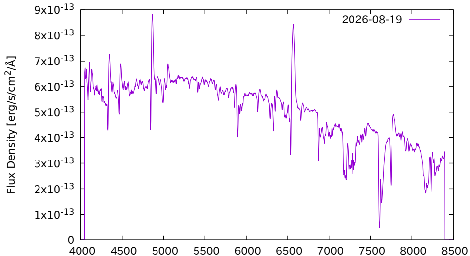
TCP J18251276-2225293 by Seimei Telescope
