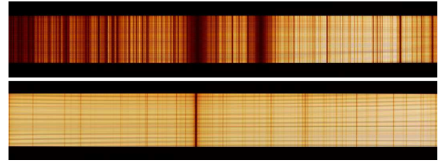
Fig. 13. Sky spectrum acquired with MIDSSAR. The prominent Ca II H&K absorption lines are clearly visible in the UV/Blue channel, while the H \alpha absorption line is detected in the Red channel. Alt text: Two detector images stacked vertically, each displaying 61 parallel, vertically aligned solar spectra with noticeable absorption features.
