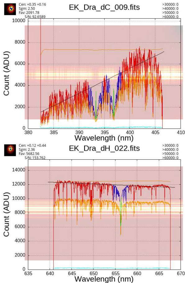
Fig. 17. Integrated data reduction summary and diagnostic display generated by the pipeline. The spectral bandpasses utilized for the automatic equivalent width calculations are plotted in distinctive colors, with the estimated continuum levels indicated by solid straight lines. To evaluate the impact of background light on the extracted spectra, the profile is co-plotted with both the absolute spectrum obtained after subtracting the average of the low-count peripheral regions and the ratio of this subtracted spectrum to the profile before subtraction. In the upper-left panel, the peak centroid position of the re-synthesized target image is highlighted in blue. For further details on the other metrics, see the main text. Alt text: For each of the two channels, the comprehensive diagnostic panel overlays the final astronomical spectrum against a faintly blended raw detector background, with a reconstructed target morphology display in the upper-left quadrant along with various quantitative observational metrics derived from the data image.
