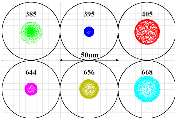
Fig. 4. Spot diagrams evaluated after the fore-optics correction. The circle indicates the physical core diameter ( 50\mu\text{m} ) of the fiber, and the numbers labeled on each spot denote the corresponding wavelengths. Depending on the relative counter-rotation angles of the ADC prisms, the centers of these spots shift from being perfectly aligned to being appropriately separated in the direction that compensates for atmospheric dispersion. Alt text: A spot diagram showing the geometric image shapes at six different wavelengths for the incident light at the center of the field of view.
