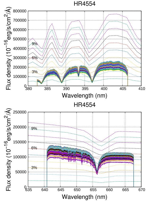
Fig. 21. Total throughput efficiency of the observation system. The observed data of HR4554 are converted to match the physical units of the spectrophotometric standard star catalog and are co-plotted within the same graphical interface. Dashed lines represent the reference catalog flux scaled by factors from 1% to 10% at increments of 1%. Note that because the spectral resolution of the reference catalog is lower than that of MIDSSAR, the profiles around strong absorption lines do not perfectly match. Alt text: Two line charts plotting the flux density on the vertical axis against wavelength on the horizontal axis, displaying the observed spectra co-plotted alongside multiple reference standard star spectra scaled by various percentage multipliers represented by dashed lines.
