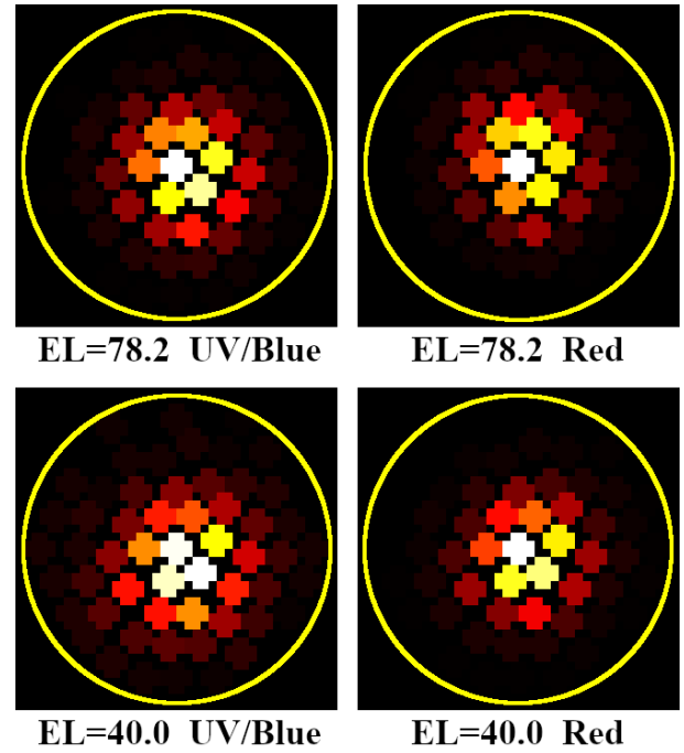
Fig. 19. Target images captured on the fiber bundle during actual science observations at different target altitudes. Upper panels: altitude angle of 78.2^\circ with integration times of 100 s (UV/Blue) and 60 s (Red). Lower panels: altitude angle of 40.0^\circ with integration times of 600 s (UV/Blue) and 300 s (Red). The circles in each panel indicate a region with a diameter of 5'' . The ADC successfully maintains the target near the center of the bundle regardless of the target altitude. Alt text: Four object images on the fiber bundle are displayed side-by-side, each surrounded by a circle indicating the 5-arcsecond diameter field.
