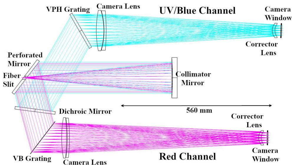
Fig. 1. Optical layout of the spectrograph main body. Light entering from the fiber slit at the left end is collimated and then divided into two wavelength bands, which are subsequently dispersed by two distinct gratings and focused by their respective camera lens systems. Alt text: An optical ray-tracing diagram showing a parabolic mirror, a perforated plane mirror, a dichroic mirror, two diffraction gratings, and two sets of camera lens systems, illustrating the specific light paths originating from the fiber slit.
