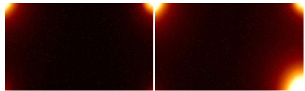
Fig. 15. Dark template images for the (left) UV/Blue channel and (right) Red channel. The parasitic background is dominated by the amp-glow component originating from the peripheral readout circuitry. Because the intensity ratios and spatial patterns of this emission vary from day to day, a combination of several distinct pre-compiled templates is utilized to dynamically synthesize and subtract the optimal dark baseline. Alt text: Two detector images placed side by side, where several of the four corners are noticeably glowing due to structured amp-glow artifacts.
