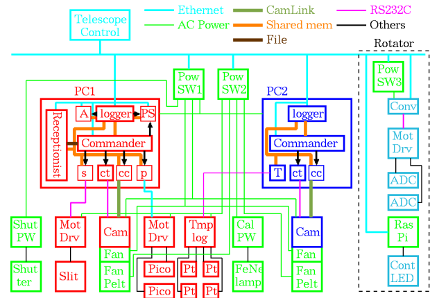
Fig. 8. System block diagram of the MIDSSAR control software. In each PC, processes enclosed by thick-lined boxes represent resident (daemon) processes, whereas those enclosed by thin-lined boxes represent processes invoked asynchronously. The abbreviations used in the diagram are defined as follows: (A) ADC control, (PS) power supply control, (s) slit position control, (ct) detector temperature control, (cc) camera exposure control, (p) fore-optics bundle positioning control, (T) instrument temperature logger, (Pow SW) network power switch, (Pelt) Peltier cooler, (Pico) Picomotor actuator, (Pt) platinum resistance thermometer, (FeNe lamp) Fe-Ne hollow cathode lamp, (Conv) Ethernet-to-RS232C converter, (Ras Pi) Raspberry Pi computer for auxiliary processing on the rotator, and (Cont LED) UV+white LED source for flat-field calibration. Alt text: A comprehensive system schematic showing all hardware and software components connected by lines that indicate their respective communication protocols.
