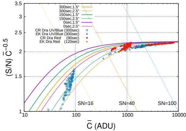
Fig. 22. Relationship between the average fiber count \bar{C} and the (S/N)\bar{C}^{-0.5} ratio. The circles and triangles represent the observation results for CR Dra and EK Dra, respectively, where open symbols denote the UV/Blue channel and filled symbols denote the Red channel. The solid curves indicate the theoretical values modeled under 1''.5 seeing (thick lines) and 2''.5 seeing (thin lines) conditions, displayed from left to right for exposure times of \sim 0 s, 150 s, and 300 s. Due to meteorological cloud attenuation, the observed data points are distributed leftward along these theoretical curves. The slanted dashed lines indicate the positions corresponding to S/N = 16 , 40, and 100 from left to right. Alt text: A scatter plot containing numerous observed data points categorized by various shapes alongside six theoretical limit curves and three vertical dashed lines, illustrating the precise correlation between the observed metrics and the modeled detection limits.
