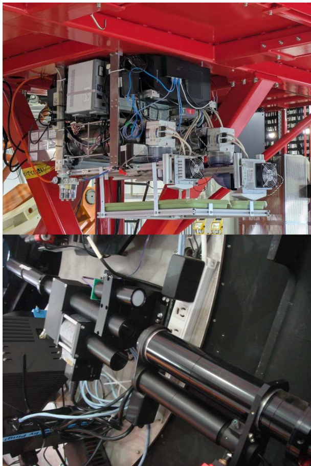
Fig. 9. Photographs of MIDSSAR mounted on the Seimei Telescope. (Top) The main body of the spectrograph installed beneath the Nasmyth platform. (Bottom) The MIDSSAR fore-optics unit mounted on the instrument rotator and positioned below the GAOES-RV fore-optics baffle. Alt text: Two photographs showing the MIDSSAR instrument components as installed on the telescope, with the upper panel displaying the spectrograph main body and the lower panel showing the fore-optics system.
