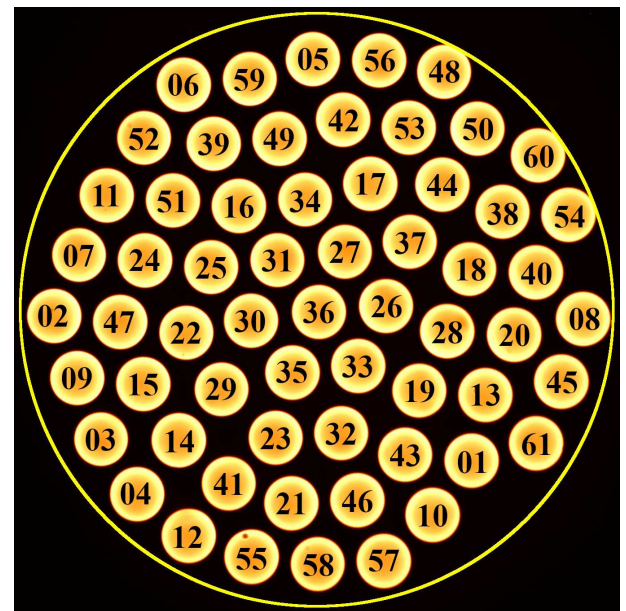
Fig. 5. Telescope-side end face of the fiber bundle. The numbers in the diagram denote the sequential index starting from the edge of the linear fiber slit on the spectrograph side, demonstrating that the fibers near the center of the slit are arranged to cluster around the center of the bundle face. The outer enclosing circle represents a physical diameter of 550\mu\text{m} , which corresponds to a 5'' field of view on the sky. Alt text: An enlarged image of the fiber bundle end face showing the arrangement of 61 individual fibers.
