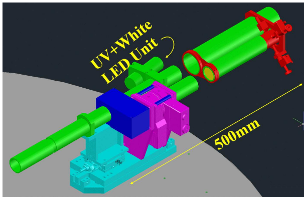
Fig. 7. Mechanical structure of the fore-optics. It is fabricated from an aluminum alloy and incorporates a commercially available \phi 30 mm lens tube and two automated rotation stages for the ADC. Rotating the instrument rotator by 8^\circ positions the LED flat-field calibration light source unit directly opposite the imaging lens. Alt text: A 3D CAD drawing showing two sets of parallel-arranged tubes integrated with two automated rotation stages on a manual translational stage.
