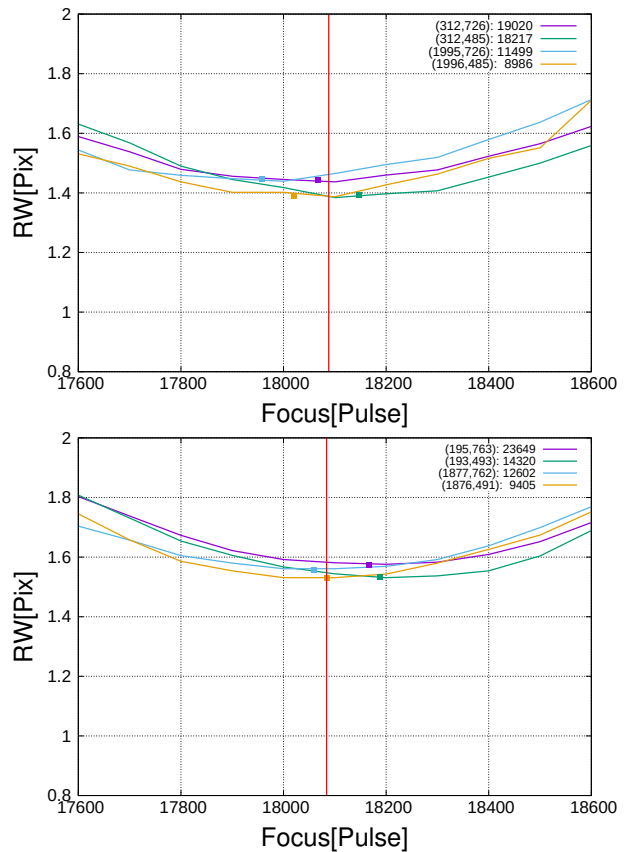
Fig. 10. Focus curves showing the spot size variation as a function of slit position displacement for four reference fiber emission line spots on the two detectors (upper panels: UV/Blue channel detector, lower panels: Red channel detector; see Figure 11 for spot locations). Small squares indicate the minimum positions derived from quadratic polynomial fits to each curve, showing that all eight spots reach minimum size at nearly identical slit positions. The red vertical dashed lines represent the overall best-focus positions determined from each detector, accounting for the relative focal offset between them. The vertical axis denotes the square root of the second-order moment of the spot profile, corresponding to a 1\sigma image radius. Both detectors achieve an optimal spot size of approximately 3 pixels, perfectly consistent with the optical design. Alt text: A plot showing two sets of four closely overlapping curves, where the minimum points for all eight curves are well-aligned near the same slit position axis.
