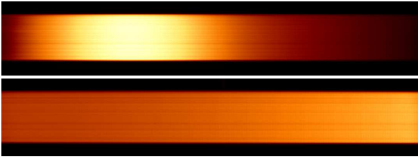
Fig. 12. Defocused LED continuum spectrum images used for flat-fielding. The upper panel displays the UV/Blue channel image capturing the emission spectrum from the UV LED, while the lower panel displays the Red channel image capturing the spectrum from the white LED. Alt text: Two detector images showing broad, belt-like continuum spectra horizontally stretching across each frame.
