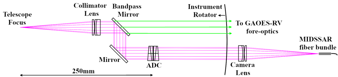
Fig. 3. Optical element layout of the MIDSSAR fore-optics system at the telescope focus. The F/6 incident beam from the telescope passes through the collimator lens and is divided by the bandpass mirror into the beam directed toward the GAOES-RV fore-optics system and the remaining wavelengths. The latter passes through the ADC and is subsequently focused by the camera lens, which is mounted on the fixed structure outside the instrument rotator, to form an image onto the fiber bundle face. Alt text: An optical ray-tracing diagram showing the layout of the collimator lens, the bandpass mirror, the counter-rotating ADC prisms, and the camera lens on the fixed structure, illustrating how the light path splits and focuses onto the fiber bundle.
