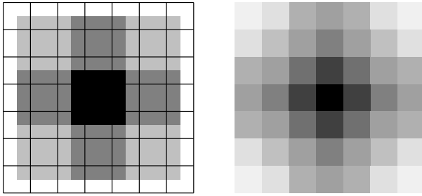
Fig. 16. Schematic diagram of the pixel subdivision process. For images where the point spread function spreads over several pixels, data values are expected to vary smoothly across adjacent pixels. Therefore, placing subpixels with intermediate values directly on the boundaries between neighboring pixels reproduces a distribution shape closer to the intrinsic physical profile. Alt text: Two side-by-side grid diagrams demonstrating pixel subdivision, showing a brightness distribution transitioning from a 3 by 3 grid to a finer 7 by 7 grid.
