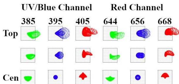
Fig. 2. Spot diagrams of the spectrograph. For the two channels, the spots represent light incident from the center, the top edge, and the intermediate position of the fiber slit, evaluated at the center and both ends of each wavelength band (wavelengths are labeled within the panels). Spots for light from the bottom half of the slit are symmetric to those from the top half. The squares indicate the size of a single pixel ( 19 \mu\text{m} ). Alt text: A spot diagram showing the geometric image shapes formed by light entering from three distinct slit positions, plotted for six different wavelengths.
