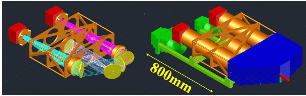
Fig. 6. Mechanical structure of the spectrograph. (Left) Internal layout showing the optical elements and light path. (Right) Entire assembled mechanical structure. The relative focal positions of the two cameras are fixed, and the global focusing of the system is executed by translationally moving the fiber slit along the optical axis. Alt text: Two 3D CAD drawings of the spectrograph: the left panel shows the internal optical layout and light path, and the right panel shows the fully assembled system with its external covers.
