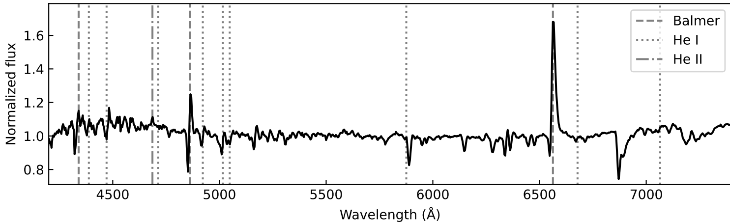
TCP J18022164-3310319 observed on 2025-03-24.990 UT with Mookodi on the Lesedi telescope at Sutherland Observatory
