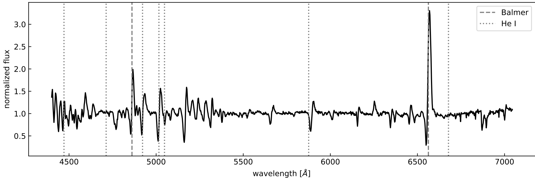
PNV J06302516-6955014 on 2025-06-06.705 UT observed with Spupnic on the 1.9m telescope at Sutherland Observatory
