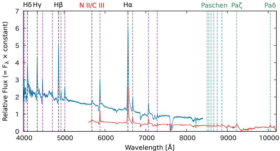
V1405 Cas = Nova Cas 2021 on 2021-03-19.41 UT (ATel #14478; Taguchi et al.) (Purple lines are He I)
