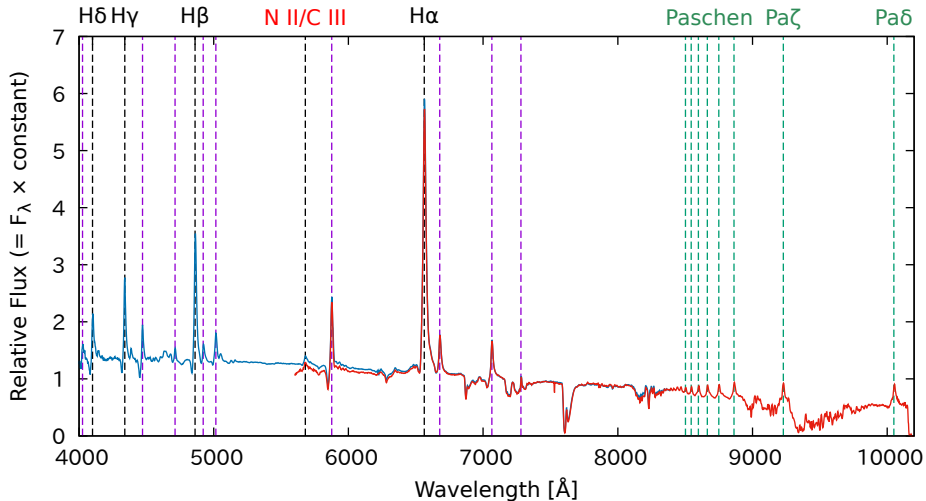
V1405 Cas = Nova Cas 2021 on 2021-03-19.84 UT (ATel #14478; Taguchi et al.) (Purple lines are He I)
