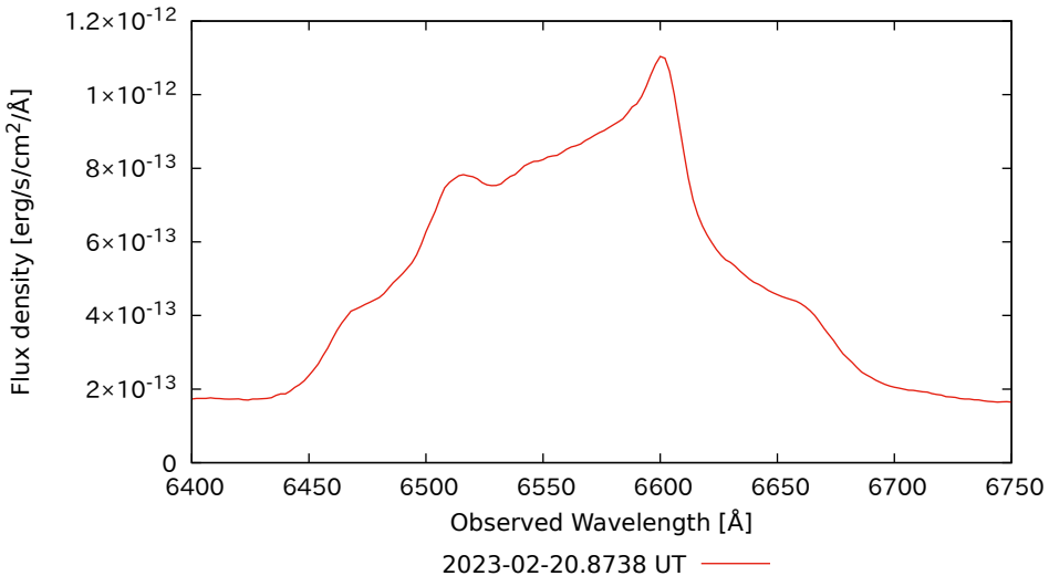
Spectrum of TCP J17562787-1714548 (Taguchi, ATel #15911)
