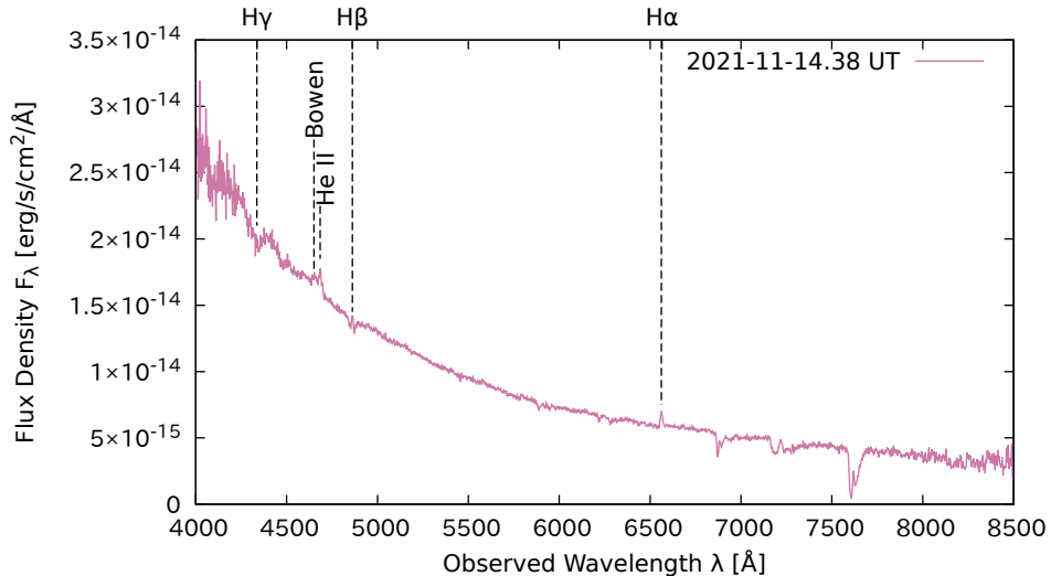
Spectrum of TCP J17242302+3258109 (Taguchi et al., ATel #15035)
