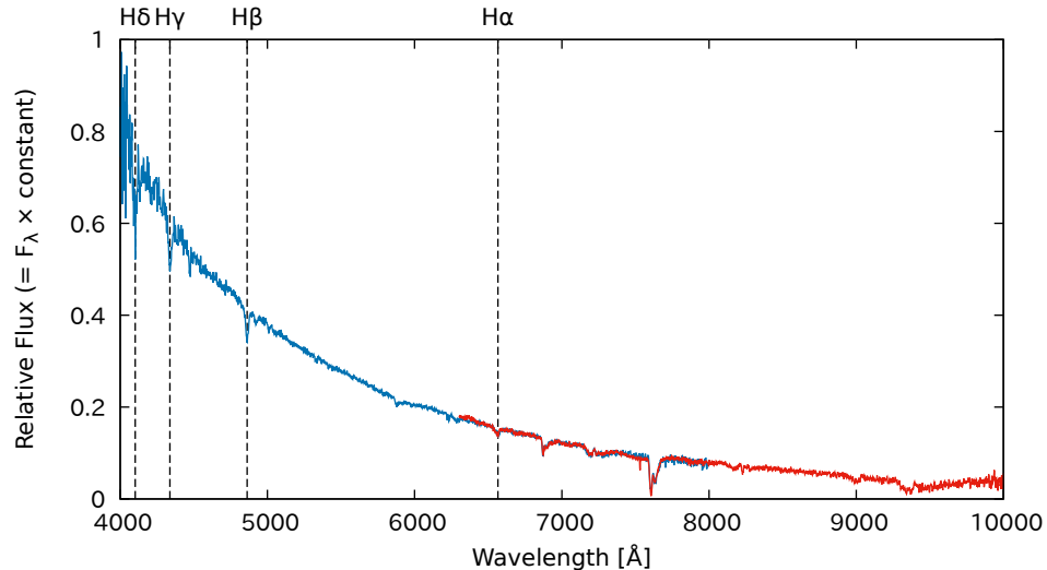
Spectrum of TCP J10203579+3103424 (Taguchi et al.)
