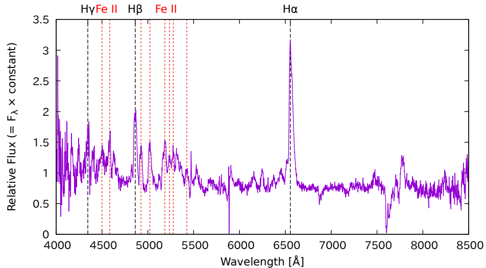
Spectrum of PNV J00425220+4116246 (Taguchi et al.)
