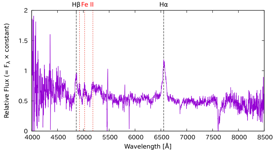
Spectrum of PNV J00434645+4122408 (Taguchi et al.)
