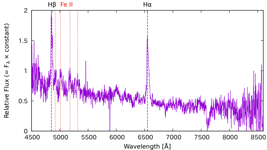
Spectrum of PNV J00420424+4042336 = AT 2021dcd (Taguchi et al.)
