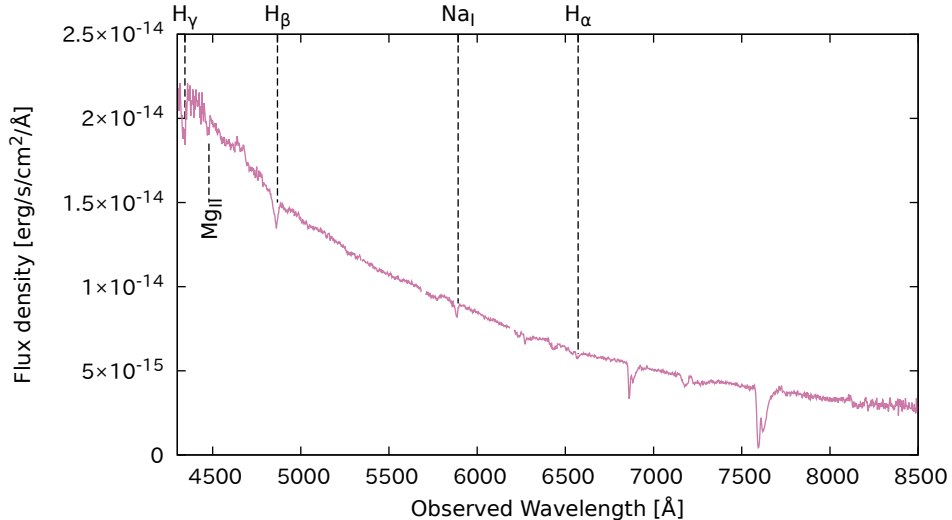
Spectrum of PNV J00215475+5231007 (Taguchi, ATel #15857)
