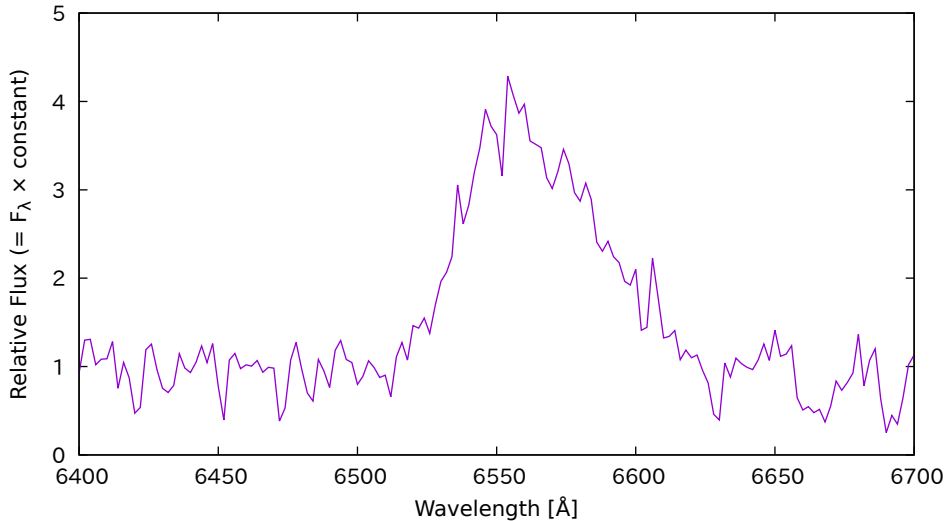
Spectrum of PNV J00434013+4127123 = AT 2021fbz (Taguchi et al.)
