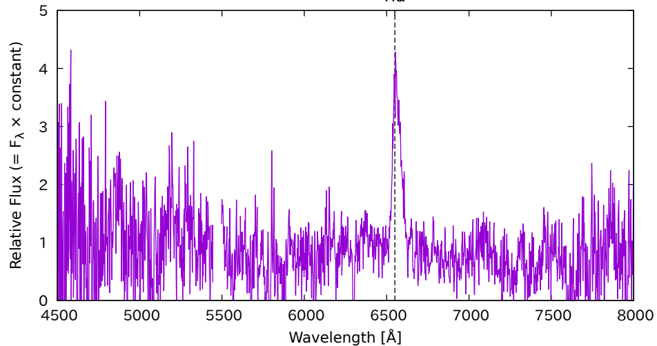
Spectrum of PNV J00434013+4127123 = AT 2021fbz (Taguchi et al.)
