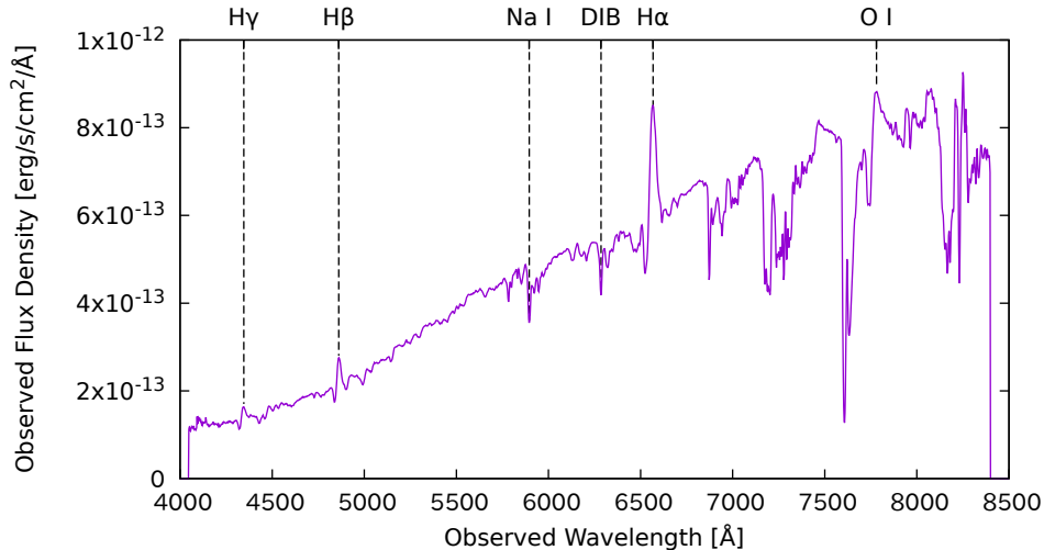
Quick Look Spectrum of PNV J19430751+2100204 by Kyoto-U. Seimei Telescope (Taguchi, ATel #16743)
