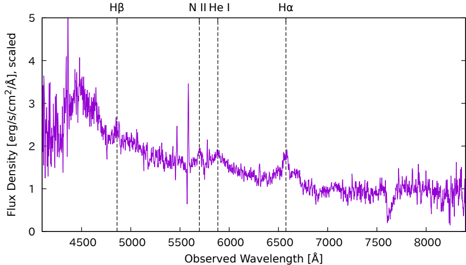
Seimei/KOOLS-IFU spectrum of M31N 2008-12a on 2025-11-30.49
