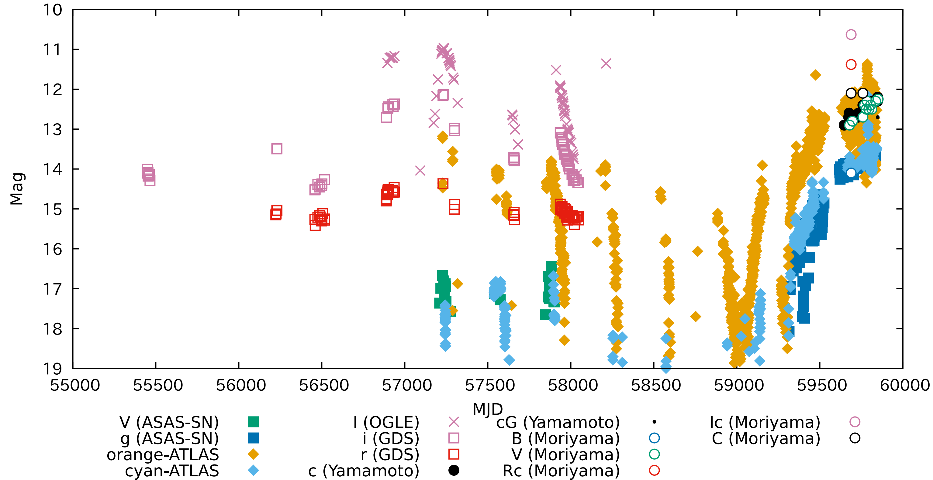
Light Curve of GDS_J1830235-135539 (Taguchi et al., ATel #15623, modified on 2022-10-03)
