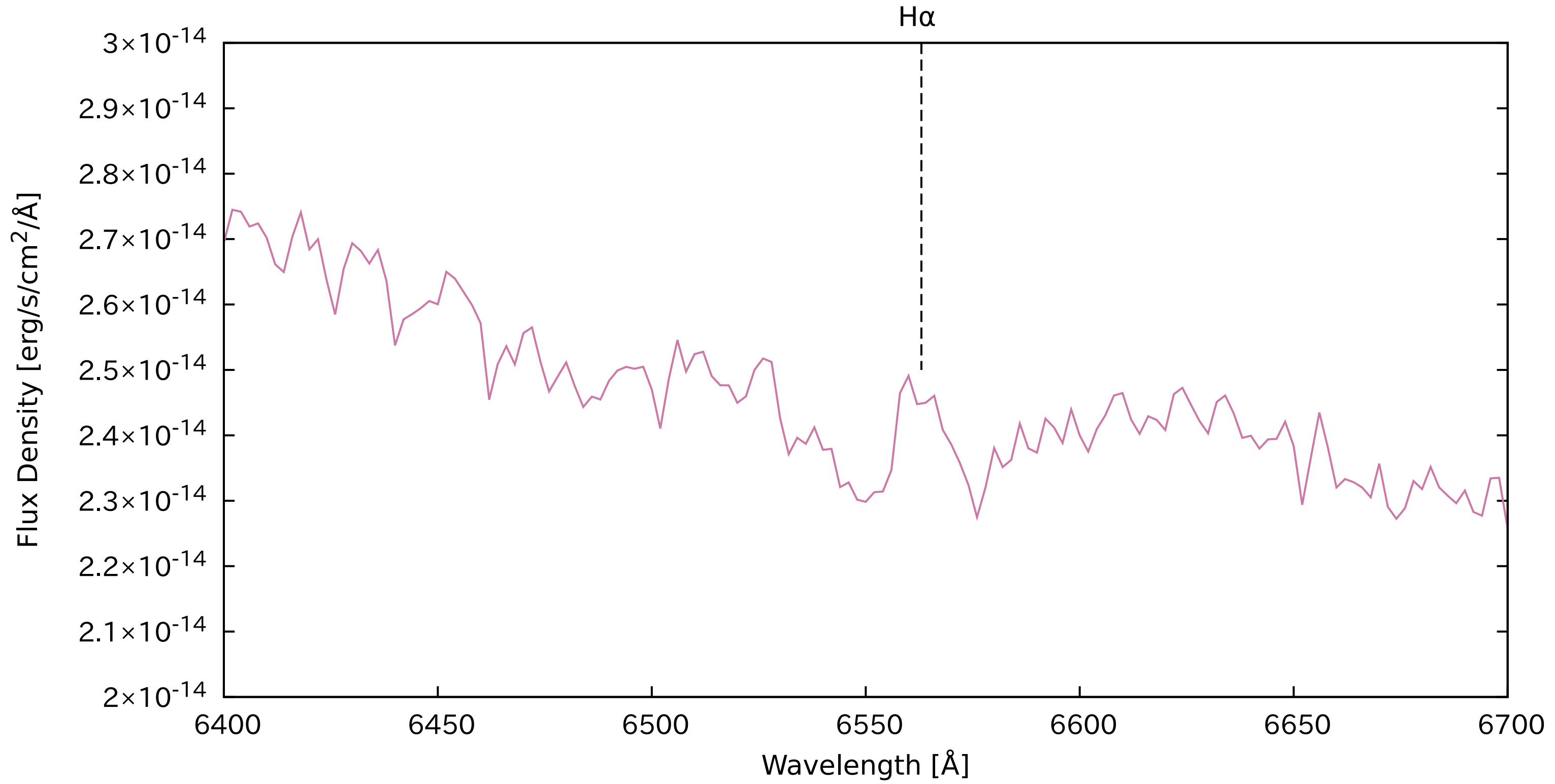
Spectrum of ASASSN-22lk by Kyoto U. Seimei Telescope (Taguchi et al., ATel #15623)
