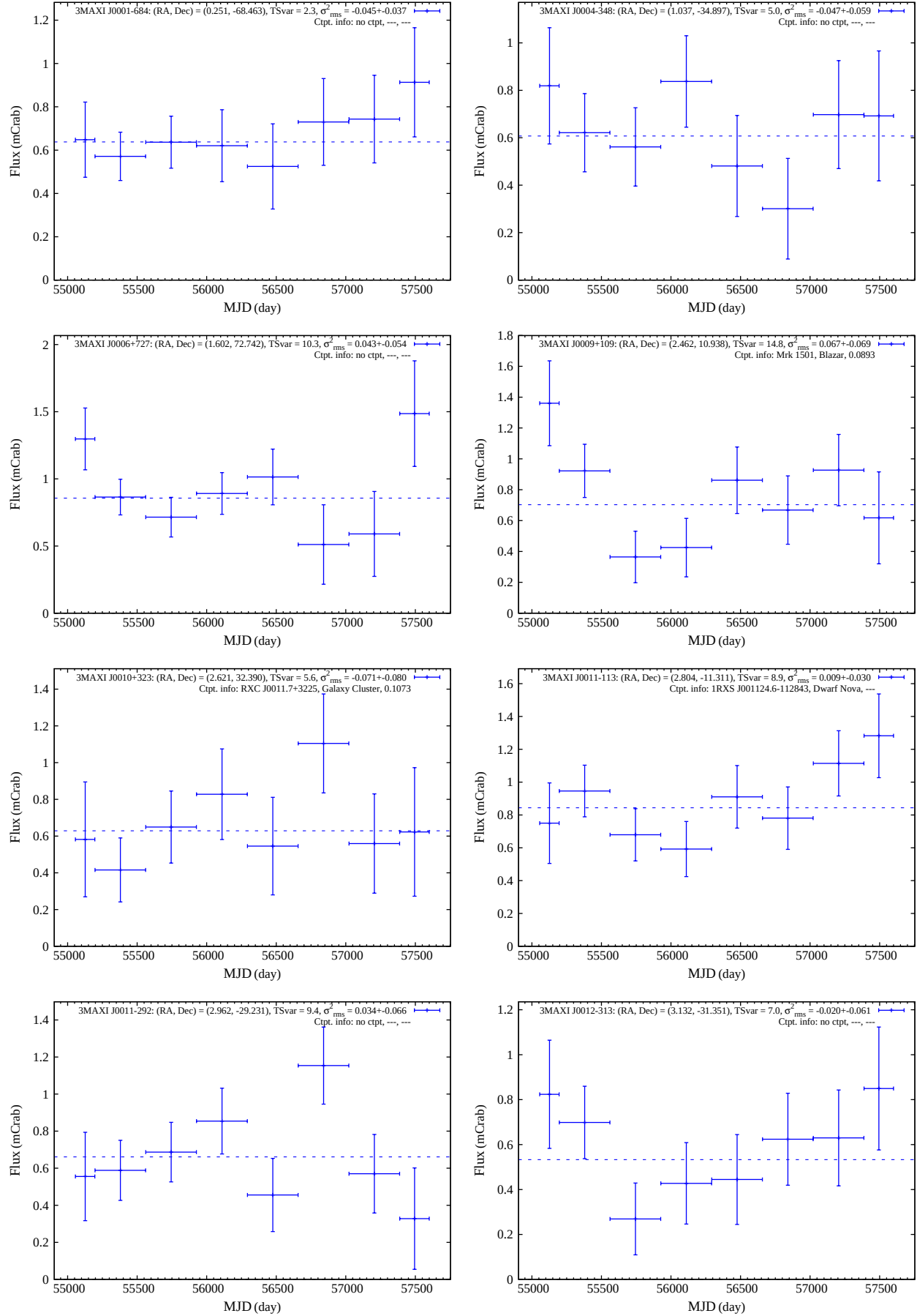
FIG. A.— Lightcurves in the 4–10 keV band during the 7 years in units of mCrab. The blue dashed line denotes the 7-year averaged flux. The counterpart information (name, type, and redshift if available) is denoted in each figure.
